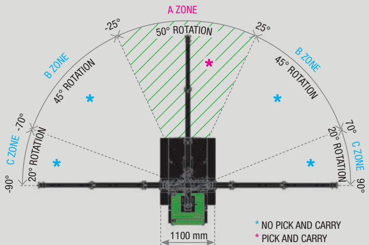
OPERATING DIAGRAM OF ROTATION WITH EXTENDED CARRIAGE
